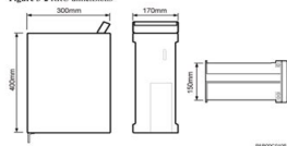
Figure 3-2 RRU dimensions
